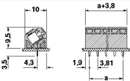
Dimensioned drawing
